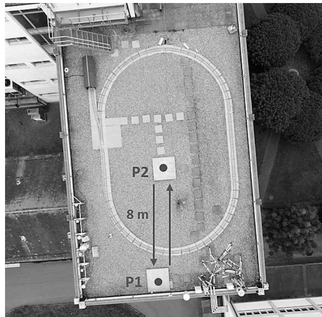
Figure 12 - RTK performance benchmarking under open sky by measuring two points alternately in the instantaneous mode for 10 minutes (Rover A vs. GS18 T, pole length: 1.800 m).
