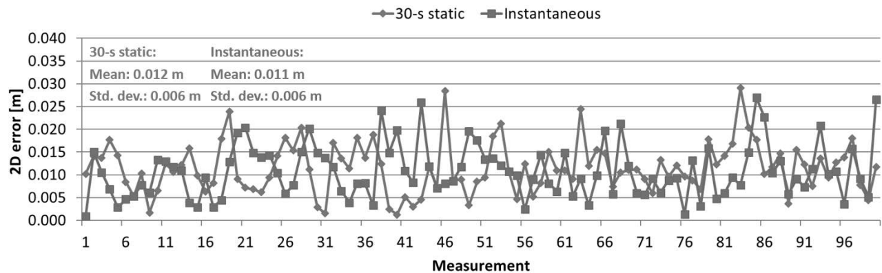
Figure 11 - Comparison of the 2D position errors from the tilt-compensated 30-s static and instantaneous measurements using the Leica GS18 T (pole length: 1.800 m, open sky; see Test 3 in Table 2).
