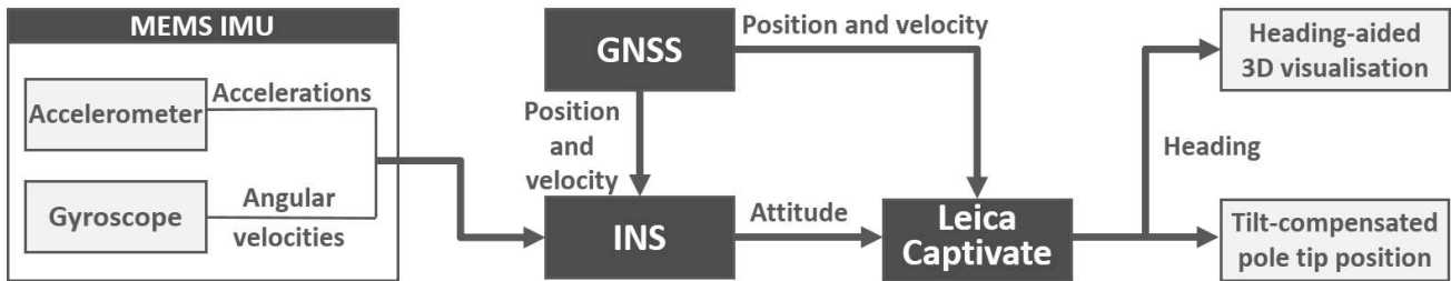
Figure 9 - Schematic and simplified illustration of the GNSS/INS integration implemented in the Leica GS18 T.
