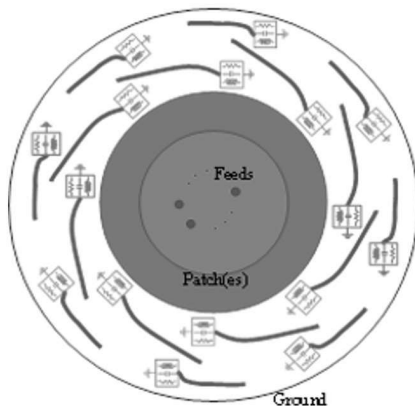
Figure 5 - Antenna concept with spiral shaped peripheral parasitic circular array loadings (Yang and Freestone, 2016).
