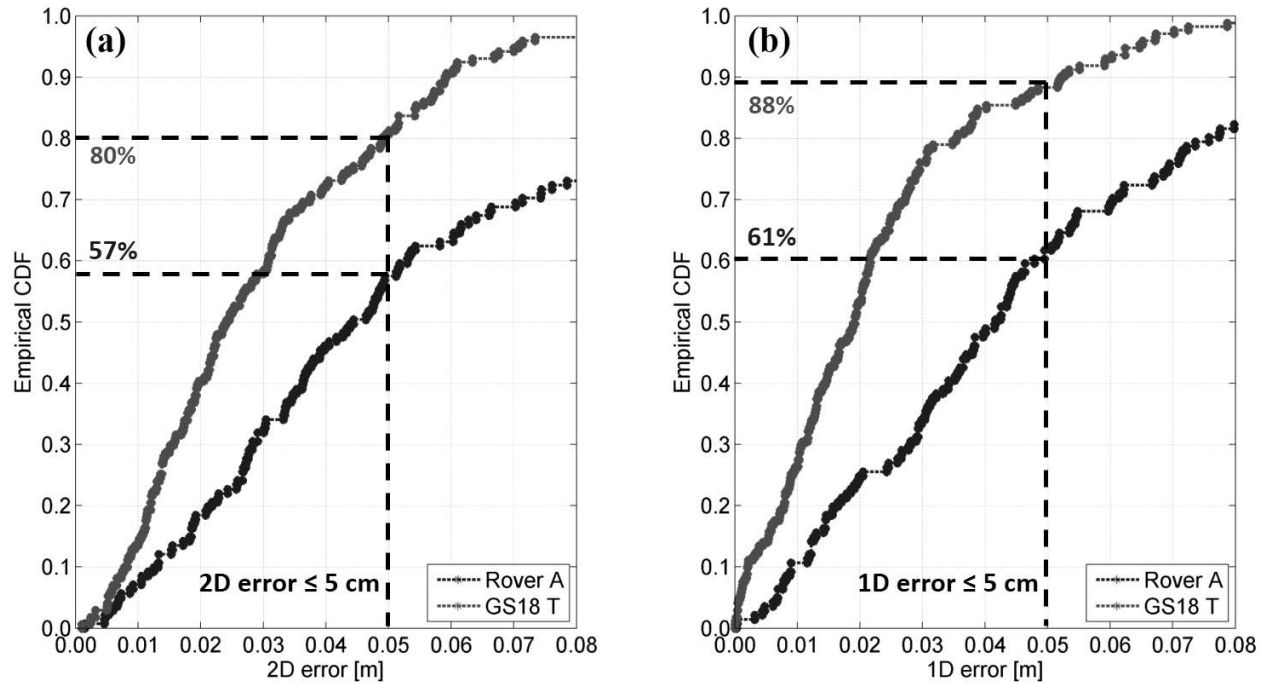
Figure 14 - Comparison of the error distributions between GS18 T and Rover A in a strong multipath environment (pole length: 1.800 m, instantaneous measurement) (a) 2D error CDF, (b) 1D error CDF.
