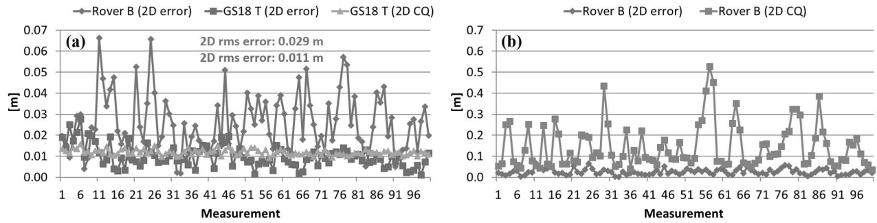
Figure 15 - Comparison of the 2D position errors and CQ between GS18 T and Rover B under magnetic disturbances (parking lot, pole length: 1.800 m, 1-s static measurement).
