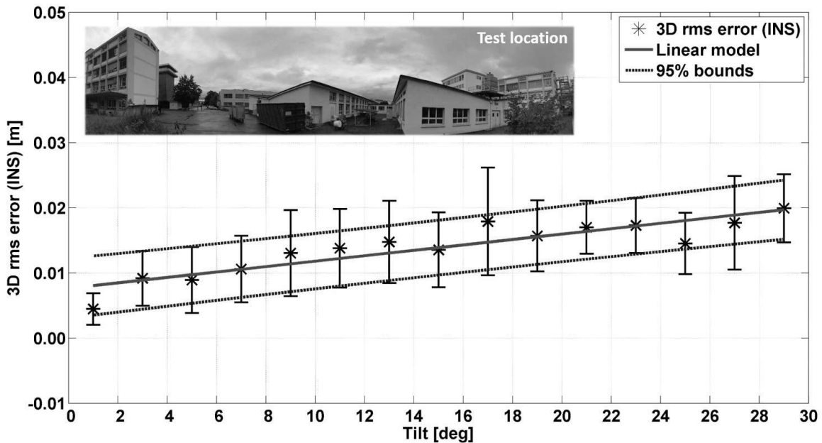
Figure 10 - 3D root mean square (rms) error of the pole tip position due to the INS attitude error by using a laser-based measurement system as a reference (pole length: 1.800 m, tilt bin width: 2 degrees).
