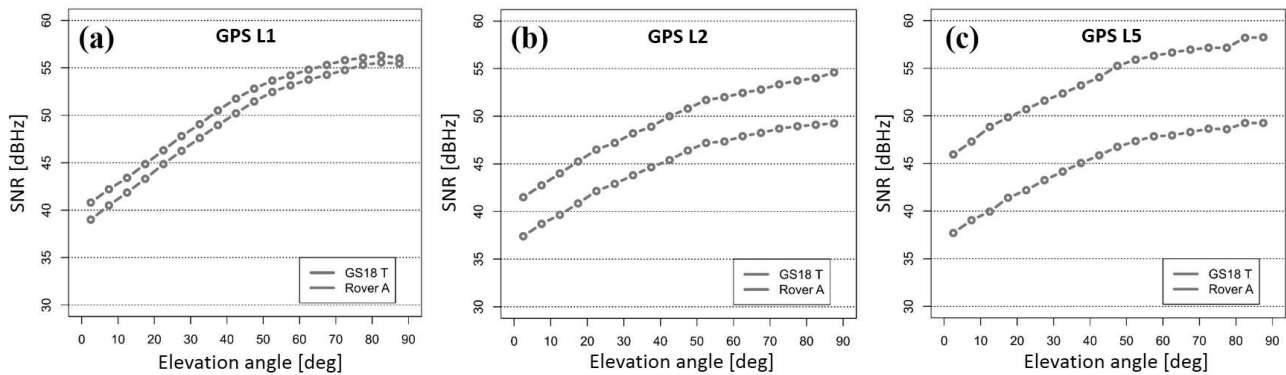
Figure 6 - Comparison of the GPS signal-to-noise ratio (SNR) measurements between GS18 T and Rover A under open sky (24 hours of 1-Hz data, elevation cut-off: 0 degrees).
