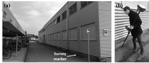
Figure 13 - RTK positioning test in a strong multipath environment (pole length: 1.800 m) (a) Survey marker near a building with metal facades, (b) Tilt compensation RTK measurement with the Leica GS18 T.
