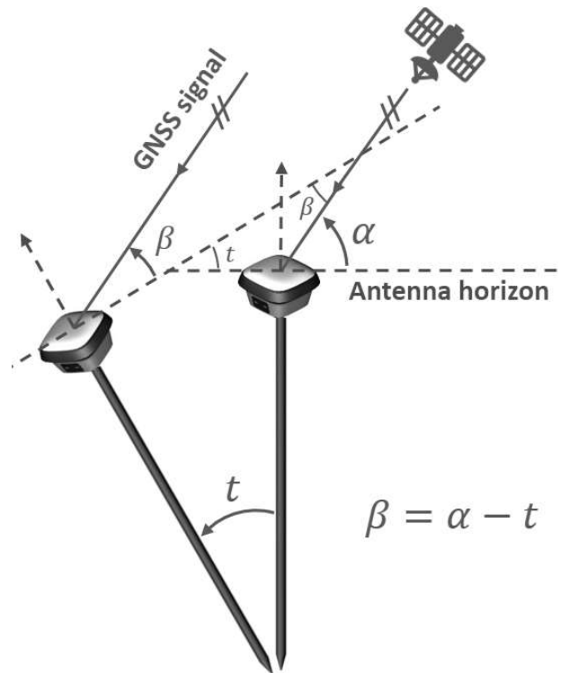
Figure 4 - Decrease in the elevation angle of the incoming GNSS signal when tilting a pole away from satellite ( \alpha asatellite elevation angle for a vertical pole, \beta : satellite elevation angle for a tilted pole, t : tilt angle).
