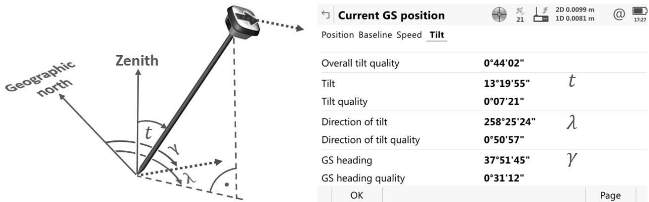
Figure 8 - Interpretation of pole attitude in the Leica GS18 T using tilt t , direction of tilt \lambda and sensor heading \gamma .
