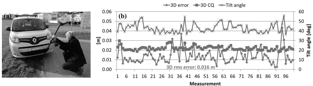
Figure 16 - 3D position errors and CQ from instantaneous measurements with large tilt angles between 36 and 56 degrees (Leica GS18 T, pole length: 1.800 m, open sky).
