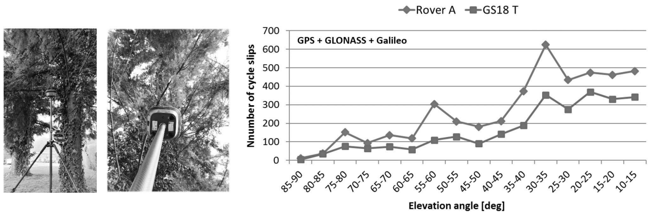
Figure 7 - Comparison of the number of cycle slips between GS18 T and Rover A under heavy tree canopy (four hours of 1-Hz data, elevation cut-off: 10 degrees).
